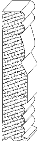
IH-500 1-5/16 x Variable base moulding
