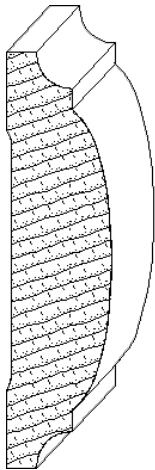
IH-379 1-1/4 x 5 chairrail_moulding
