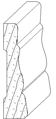
IH-498 1/2 x 2-1/4 casing moulding
