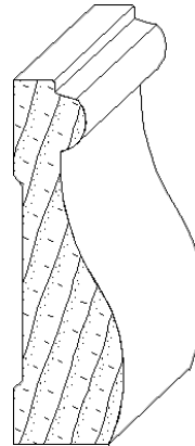
IH-1461 3/4 x 2-1/2 casing moulding
