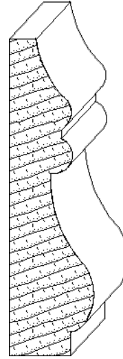
IH-14004 1-1/4 x 4-11/16 casing moulding
