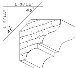
IH-1605 3/4 x 1-3/4 crown_moulding
