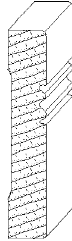
IH-330 3/4 x 4 chairrail_moulding
