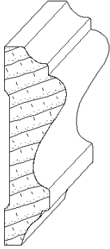
IH-381 3/4 x 2-3/8 chairrail_moulding
