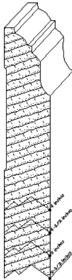
IH-557 1 x Variable base moulding
