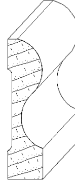
IH-368 1/2 x 2 chairrail_moulding
