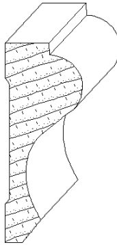
IH-301 1-1/16 x 2-3/4 chairrail_moulding
