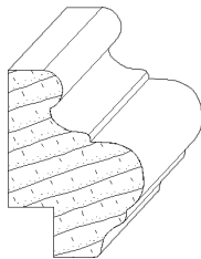
IH-535 1-3/16 x 1-5/8 base moulding
