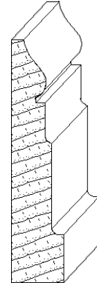
IH-1495 3/4 x 3-1/2 casing moulding
