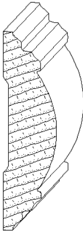
IH-347 1 x 3-3/4 chairrail_moulding
