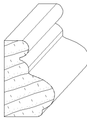
IH-590 3/4 x 1-1/8 base moulding
