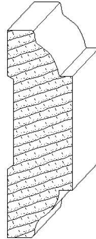
IH-341 1-1/4 x 4 chairrail_moulding
