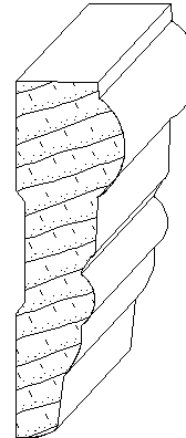
IH-369 3/4 x 2-1/4 chairrail_moulding
