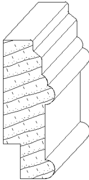
IH-377 3/4 x 2 chairrail_moulding
