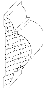
IH-317 1-1/8 x 2-7/8 chairrail_moulding
