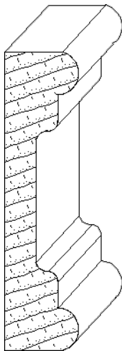
IH-398 7/8 x 3-1/2 chairrail_moulding
