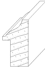
IH-269 3/4 x 1-3/8 cabinet moulding
