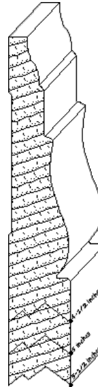
IH-566 1 x Variable base moulding
