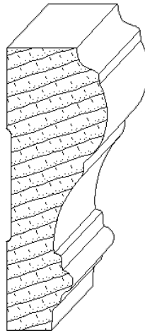
IH-319 1-1/4 x 3-1/2 chairrail_moulding
