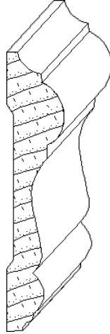
IH-351 5/8 x 3 chairrail_moulding
