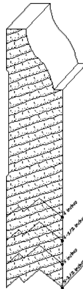
IH-562 1-13/16 x Variable base moulding
