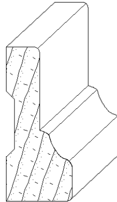
IH-1411 3/4 x 1-3/4 casing moulding
