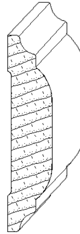
IH-334 3/4 x 3-1/4 chairrail_moulding
