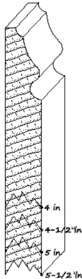
IH-1572 13/16 x variable base moulding
