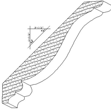
IH-689 1 x 7-3/4 crown_moulding
