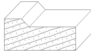
IH-227 1 x 2-1/4 cabinet moulding
