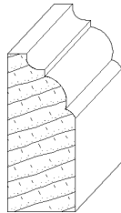
IH-1589 3/4 x 1-3/4 base moulding
