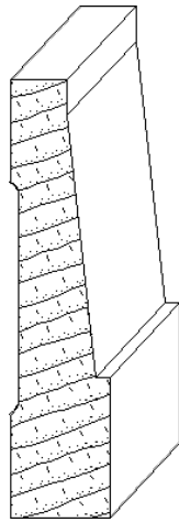
IH-343 3/4 x 3-1/4 chairrail_moulding
