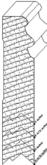
IH-523 1-3/16 x Variable base moulding
