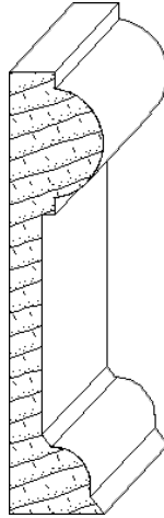
IH-382 3/4 x 3-1/2 chairrail_moulding
