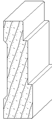
IH-484 3/4 x 2-1/2 casing moulding
