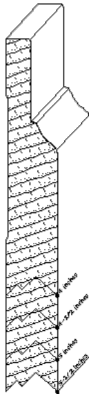
IH-518 13/16 x Variable base moulding
