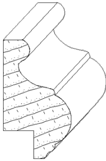
IH-358 1 x 1-3/4 chairrail_moulding
