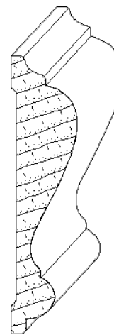
IH-324 3/4 x 3-1/8 chairrail_moulding
