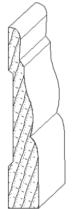
IH-1448 5/8 x 3-3/4 casing moulding
