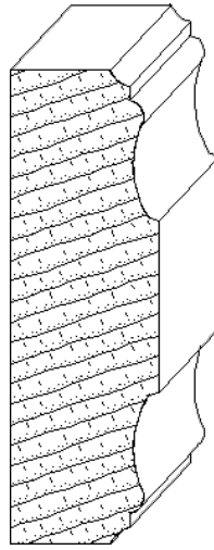
IH-395 1-1/4 x 4 chairrail_moulding
