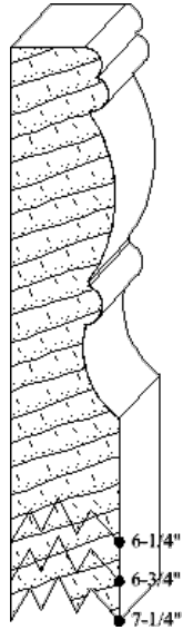
IH-1580 1-3/8 x variable base moulding
