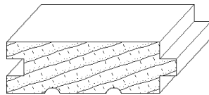
IH-800 (Face) 3/4 x 2-1/4 flooring
