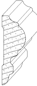
IH-353 7/8 x 2-1/2 chairrail_moulding
