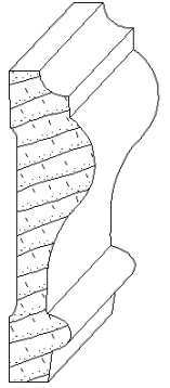
IH-305 5/8 x 2-1/2 chairrail_moulding
