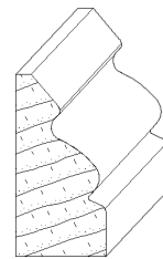
IH-584 3/4 x 1-9/16 base moulding
