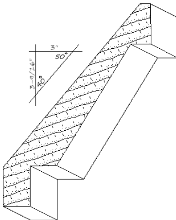
IH-1616 7/8 x 4-5/8 crown_moulding
