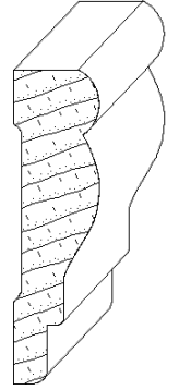
IH-332 11/16 x 2-1/2 chairrail_moulding
