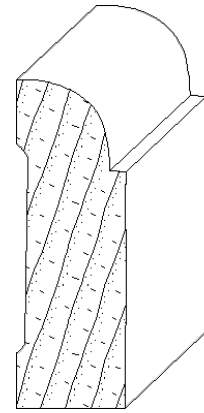
IH-425 3/4 x 2-1/4 casing moulding
