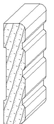
IH-414 9/16 x 2-5/8 casing moulding
