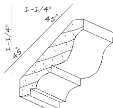
IH-687 3/8 x 1-3/4 crown_moulding
