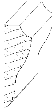
IH-383 5/8 x 1-7/8 chairrail_moulding
