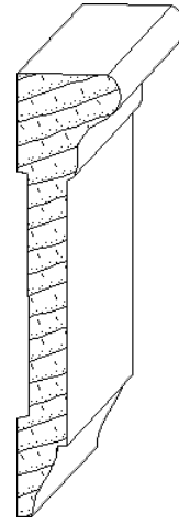
IH-346 13/16 x 3-1/2 chairrail_moulding
